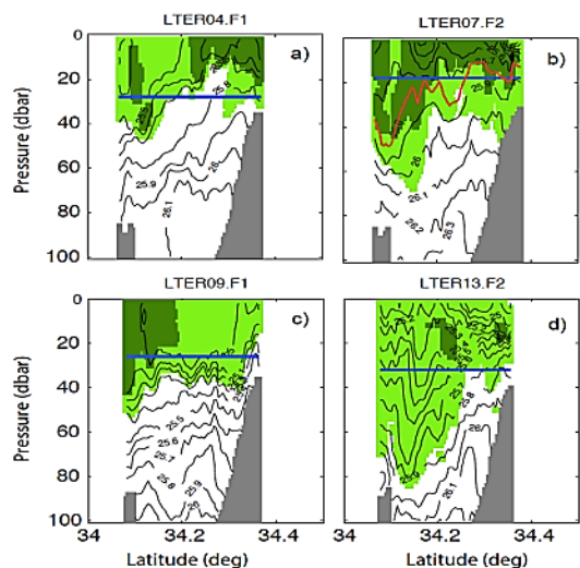
Fig. 12. Sections across the SBC of potential density anomaly \sigma_\theta in \text{kg m}^{-3} (black lines) and chlorophyll concentrations ( > 1 \text{ mg m}^{-3} light green; > 5 \text{ mg m}^{-3} dark green) from 4 cruises. Horizontal blue lines show 1% light depths.
